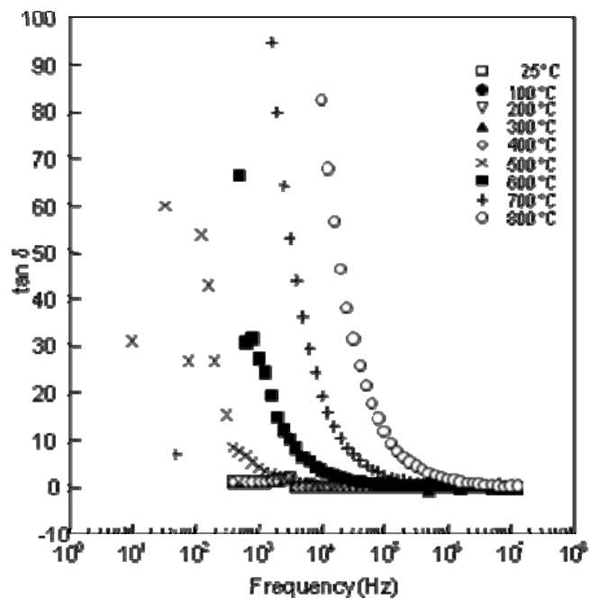
Figure 6: Dielectric loss, \tan \delta of \text{Bi}_3\text{Mg}_2\text{Nb}_3\text{O}_{14} as a function of frequency at different temperatures
