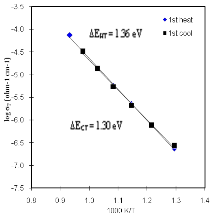
Figure 9: Conductivity Arrhenius plot of \text{Bi}_3\text{Mg}_2\text{Nb}_3\text{O}_{14} sintered at 1025^\circ\text{C}
