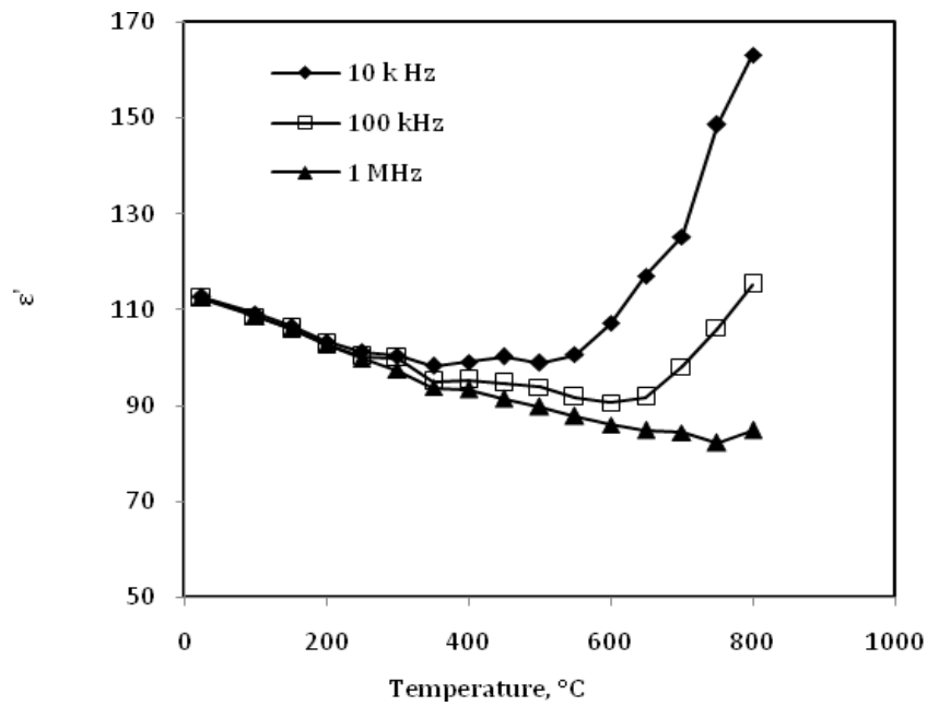
Figure 3: Dielectric constant, \epsilon' of \text{Bi}_3\text{Mg}_2\text{Nb}_3\text{O}_{14} as a function of temperatures at different frequencies
