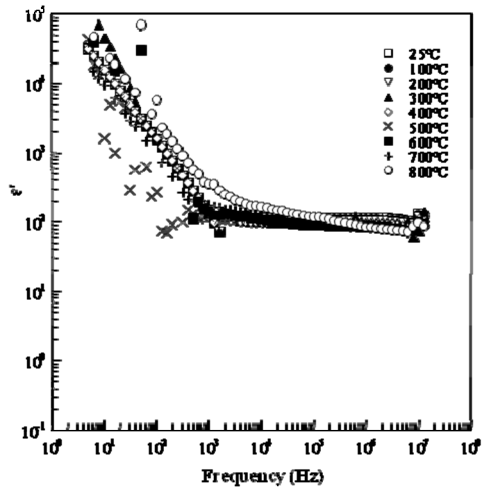
Figure 5: Dielectric constant, \epsilon' of \text{Bi}_3\text{Mg}_2\text{Nb}_3\text{O}_{14} as a function of frequency at different temperatures
