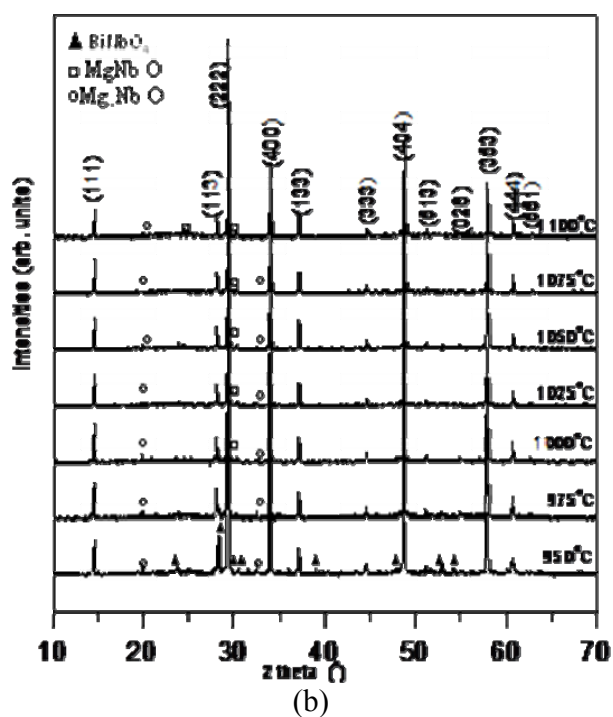
Figure 1: X-ray diffraction patterns for the \text{Bi}_3\text{Mg}_2\text{Nb}_3\text{O}_{14} annealed at (a) 800°C to 925°C and (b) 950°C to 1100°C
