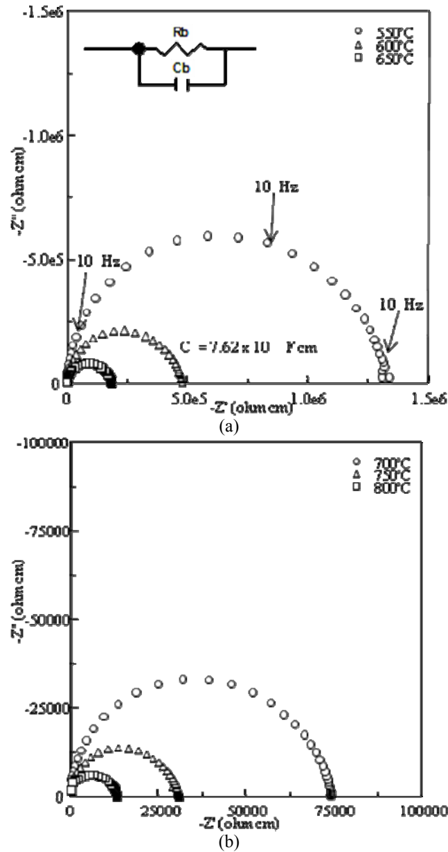
Figure 7: Complex plots of \text{Bi}_3\text{Mg}_2\text{Nb}_3\text{O}_{14} at different temperatures
