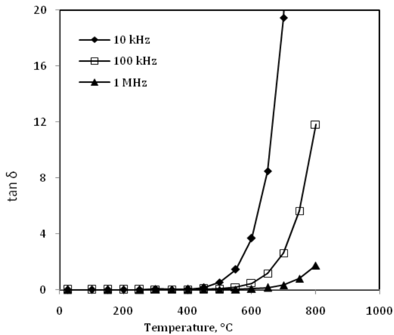
Figure 4: Dielectric loss, \tan \delta of \text{Bi}_3\text{Mg}_2\text{Nb}_3\text{O}_{14} as a function of temperatures at different frequencies
