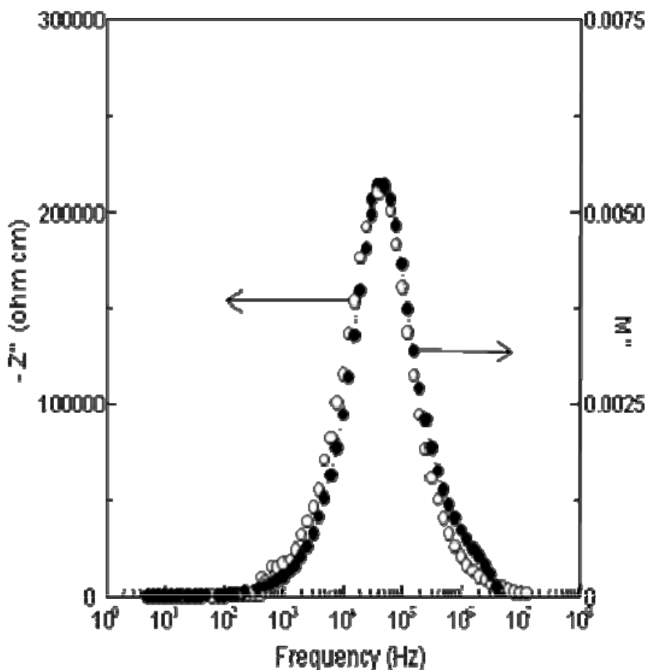
Figure 8: Combined spectroscopic plot of \text{Bi}_3\text{Mg}_2\text{Nb}_3\text{O}_{14} at 650^\circ\text{C}
