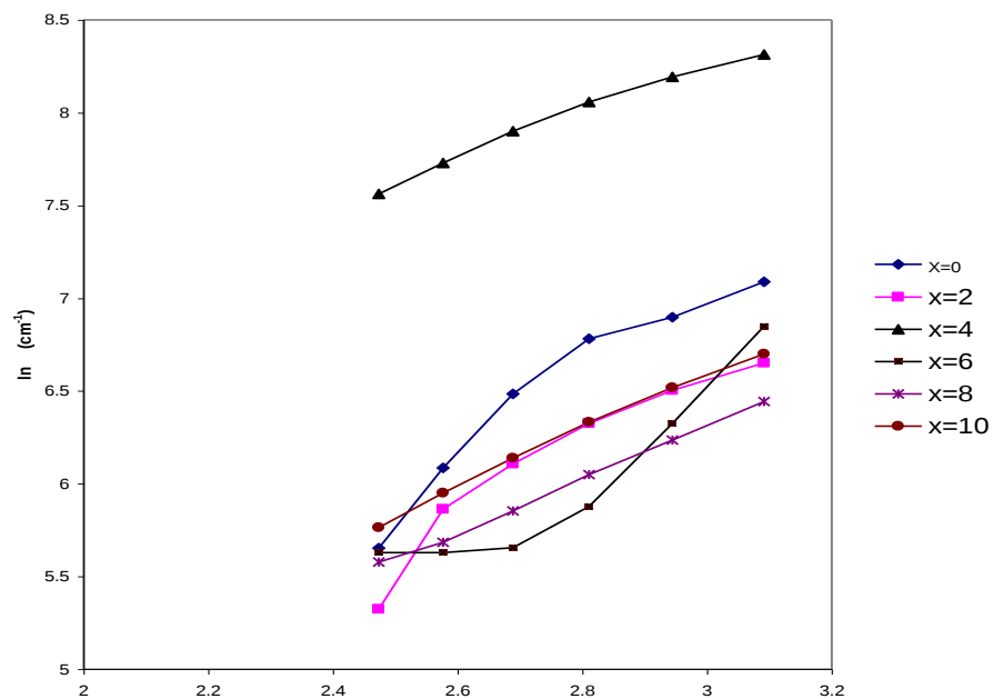
Figure 2: The \ln \alpha versus \hbar\omega for various \text{Nd}_2\text{O}_3 (mol%) content for x\text{Nd}_2\text{O}_3-(35-x)\text{CuO}-65\text{P}_2\text{O}_5 system
