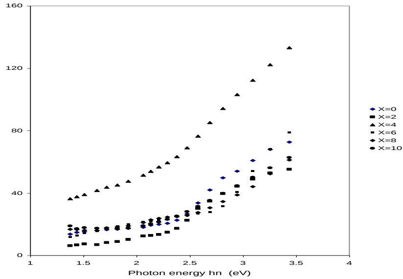
Figure 1: (\alpha\hbar\omega)^{1/2} versus \hbar\omega for various \text{Nd}_2\text{O}_3\text{-CuO-P}_2\text{O}_5 glasses
