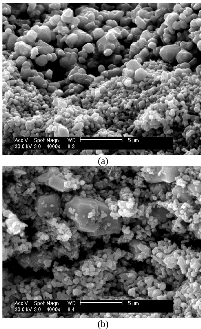
Figure 3: SEM micrographs of fractured surface (a) CuO/ZnO, and (b) 97CuO-3Al 2 O 3 /ZnO samples.
