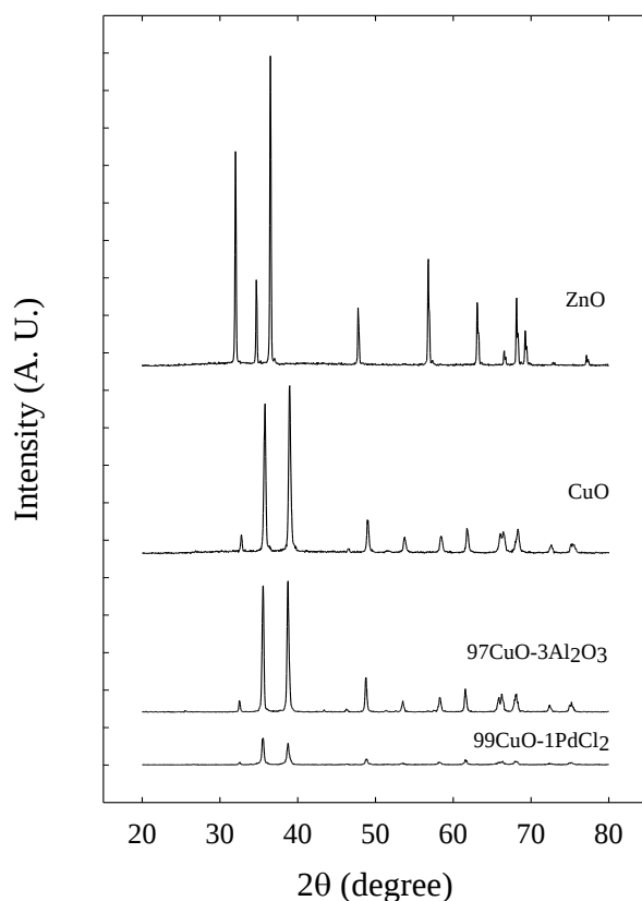
Figure 2: Powders XRD patterns of \text{ZnO} , \text{CuO} , 97\text{CuO}-3\text{Al}_2\text{O}_3 and 99\text{CuO}-1\text{PdCl}_2 samples calcined at 800^\circ\text{C} for 3 h.
