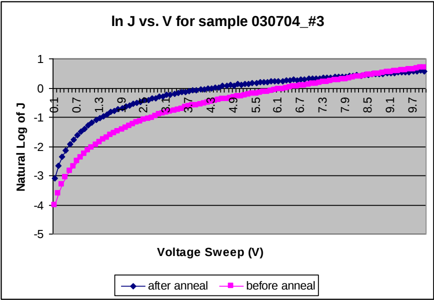
Figure 3: Current density vs voltage plot for sample 030704_#3
