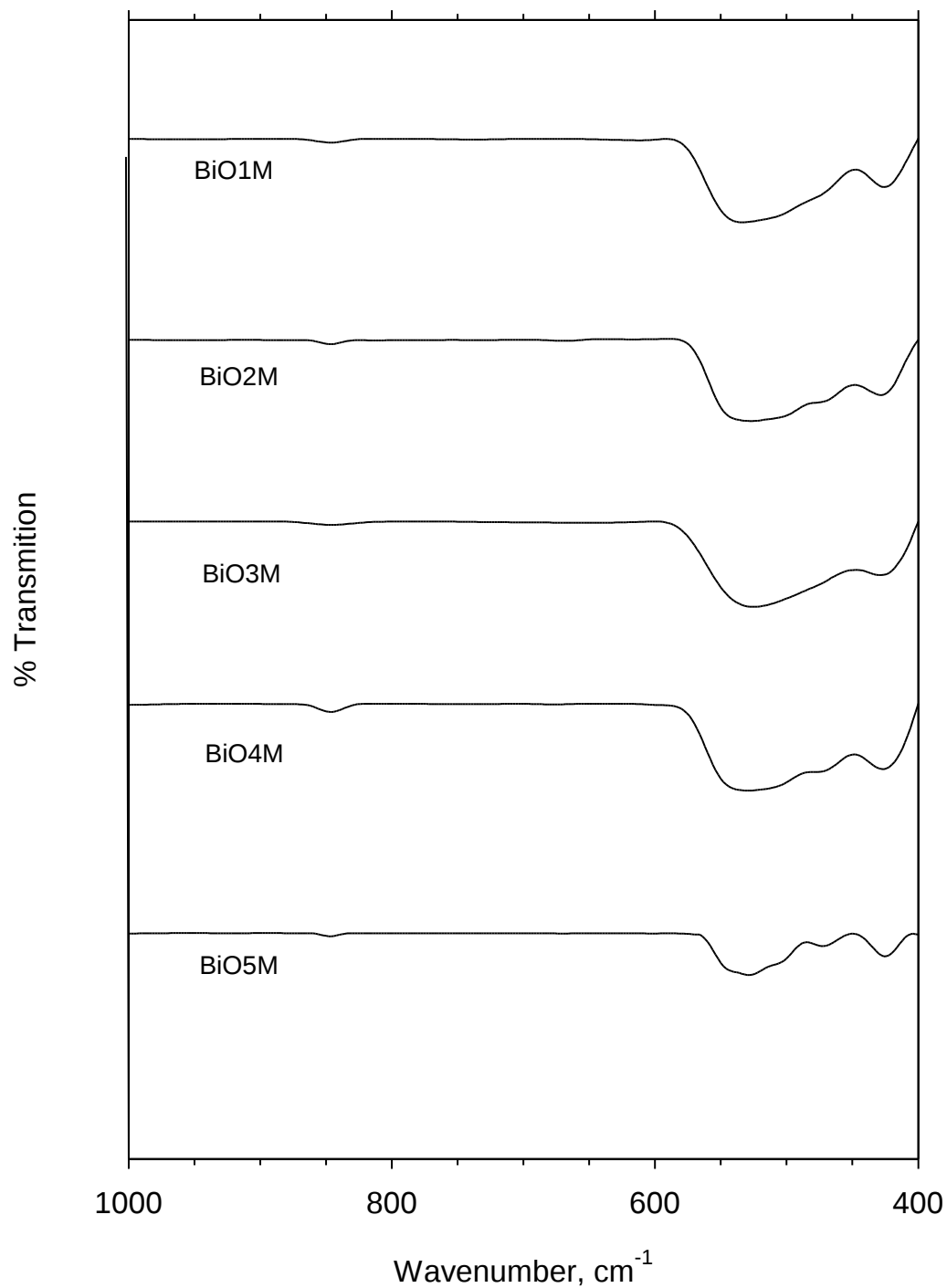
Figure. 5: FT-IR spectrum of BiO1M, BiO2M, BiO3M, BiO4M and BiO5M samples
