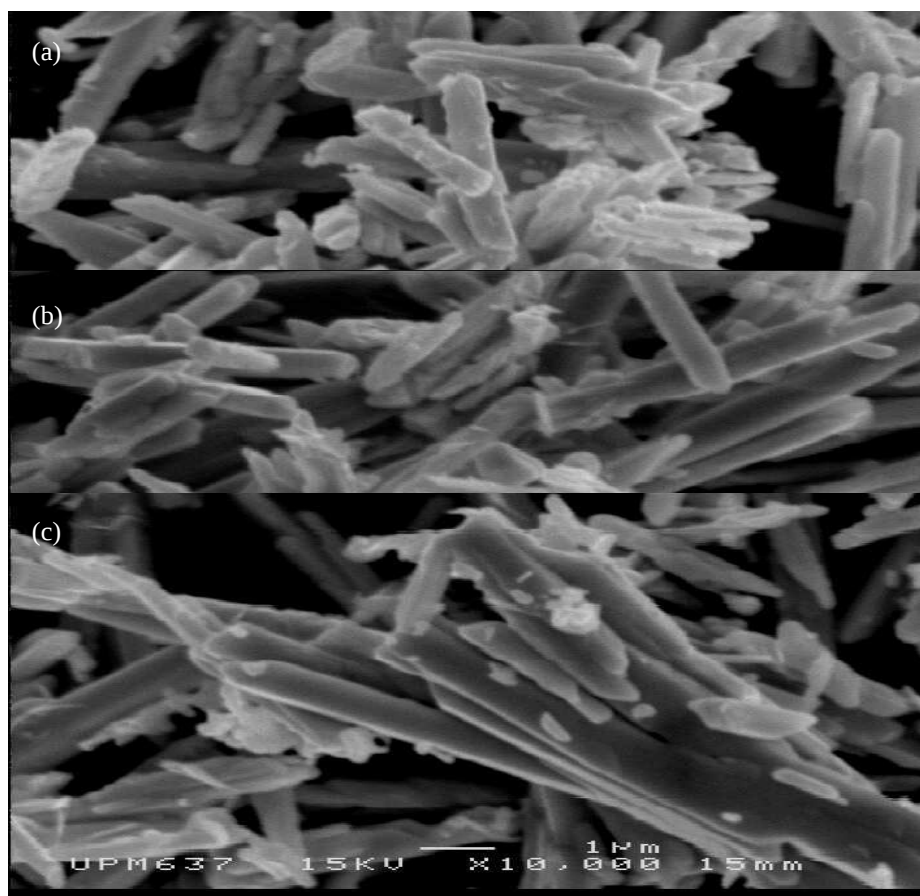
Figure. 6: SEM image of samples a) BiO1M b) BiO3M c) BiO5M (x10,000)
