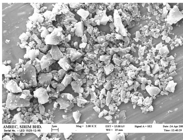
Figure 5: SEM micrograph of RH3 carbon electrode a)before and b) after milling process
