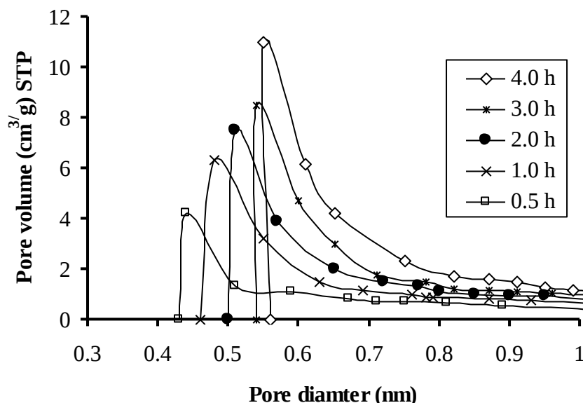
Figure 5: the influence of activation times in the pore development.
