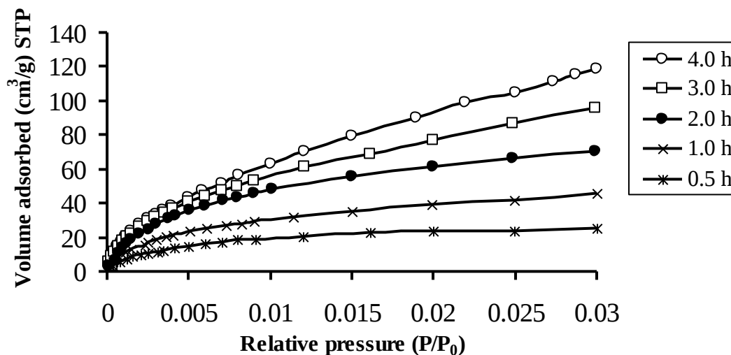
Figure 2: CO 2 adsorption isotherms of activated carbon at different activation time.
