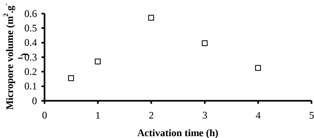
Figure 3: Micropore volume of activated carbon at different activation time.
