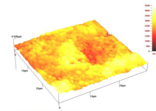
X=0.10 Average grain size: 2.10μm
