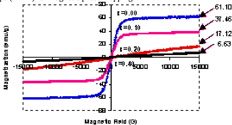
Figure 3: Hysteresis loops of (\text{La}_{1-x}\text{Dy}_x)\text{Sr}_{0.33}\text{MnO}_3 compound with x=0.00, 0.10, 0.20 and 0.40 .
