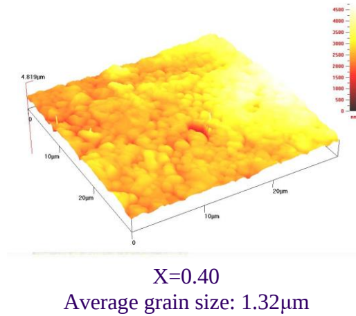
Figure 2: AFM images for (a) x=0.00 , (b) x=0.10 , x=0.20 and (c) x=0.40 .
