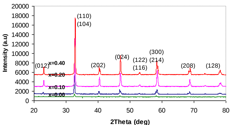
Figure 1: X-ray diffraction (XRD) patterns of (\text{La}_{1-x}\text{Dy}_x)\text{Sr}_{0.33}\text{MnO}_3 compound with x=0.00, 0.10, 0.20 and 0.40 .
