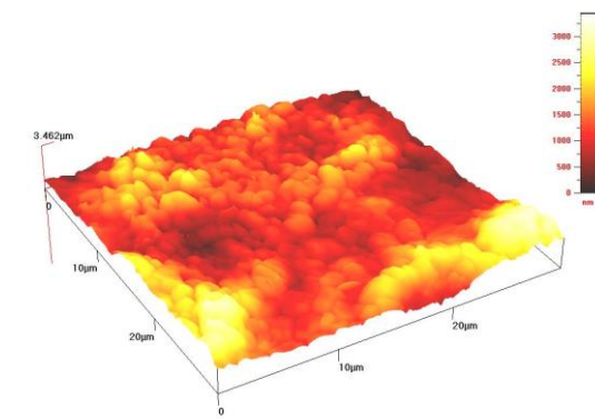
X=0.00 Average grain size: 2.24μm
