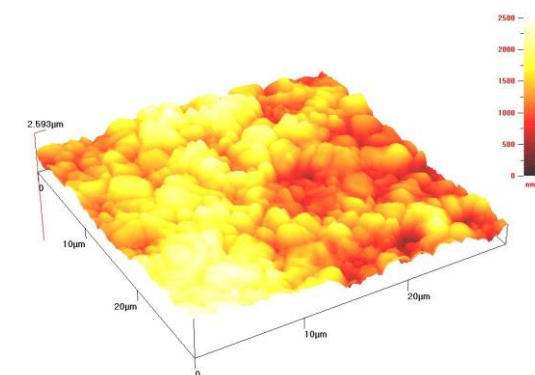
X=0.20 Average grain size: 1.80μm
