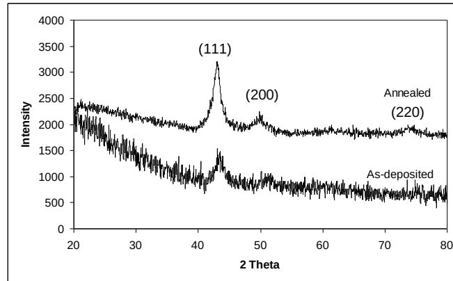
Figure 3 : XRD pattern for as-deposited and annealed CuCo film at 300°C for 15 minutes
