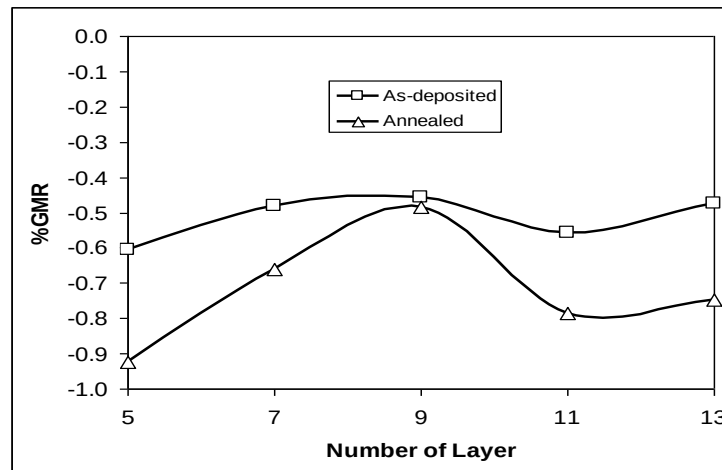
Figure 6: Giant magnetoresistance value of as-deposited and annealed sample at different layer
