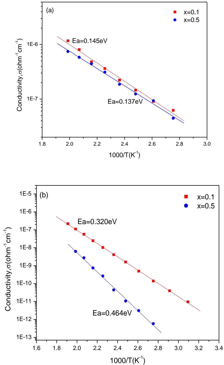
Figure 5: Arrhenius plot of (a) bulk conductivity and (b) grain boundary conductivity of \text{Ca}_{1-x}\text{Sr}_x\text{Cu}_3\text{Ti}_4\text{O}_{12} ( x = 0.1 and 0.5 ) ceramics sintered at 1050 °C.
