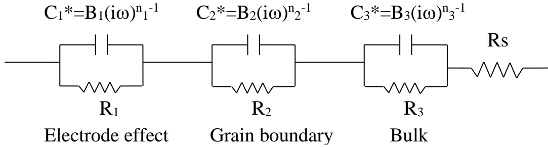
Figure 4: Equivalent circuit used to model the \text{Ca}_{1-x}\text{Sr}_x\text{Cu}_3\text{Ti}_4\text{O}_{12} response.
