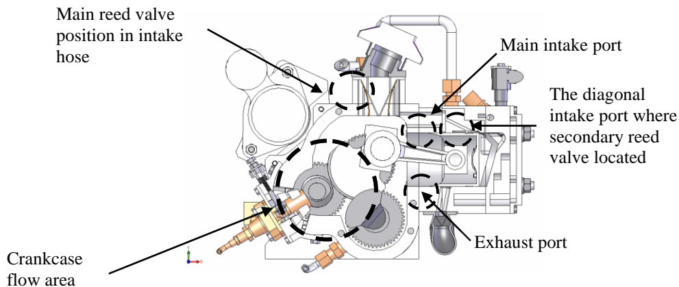
Figure 1: Cut view of the two stroke diesel.
