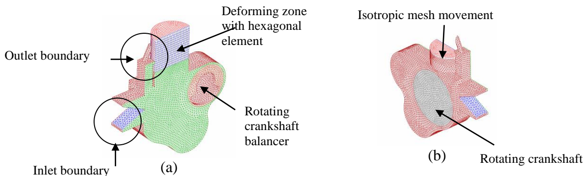
Figure 2(a) and 2(b): Meshed model using hexahedral and tetrahedral element and description of moving and stationary parts and boundary.
