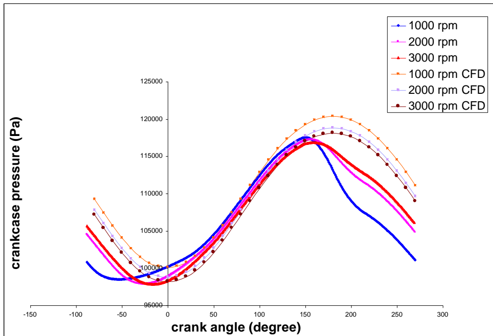
Figure 5: Crankcase pressure measured at 1000, 2000 and 3000 rpm and calculated crankcase pressure at same engine speed without pre-defined exhaust and intake pressure boundary (all valves closed).
