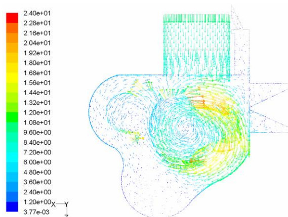
Figure 6: Vectors of velocity magnitude at 70 CA after to dead centre (ATDC) at 3000 rpm.
