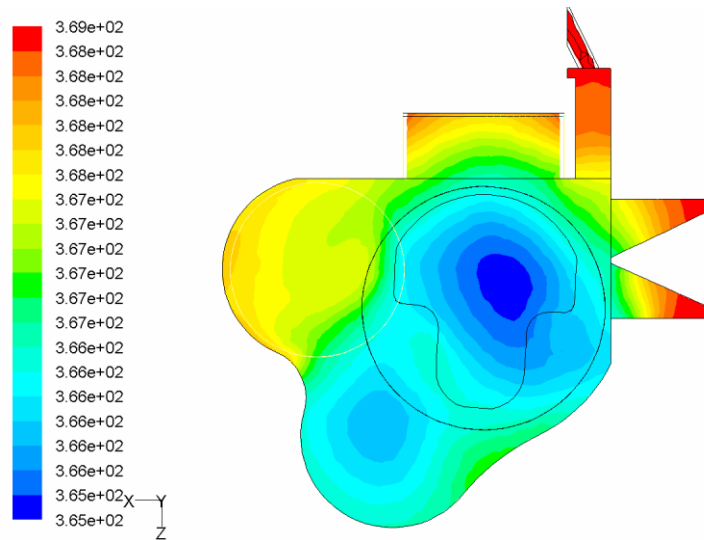
Figure 7: contours of static temperature at 180 CA ATDC at 3000 rpm.
