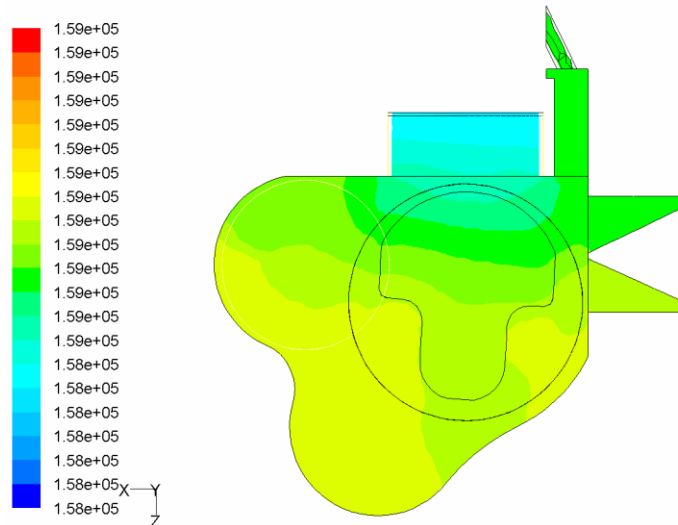
Figure 8: Contours of static pressure at 180 CA ATDC at 3000 rpm.
