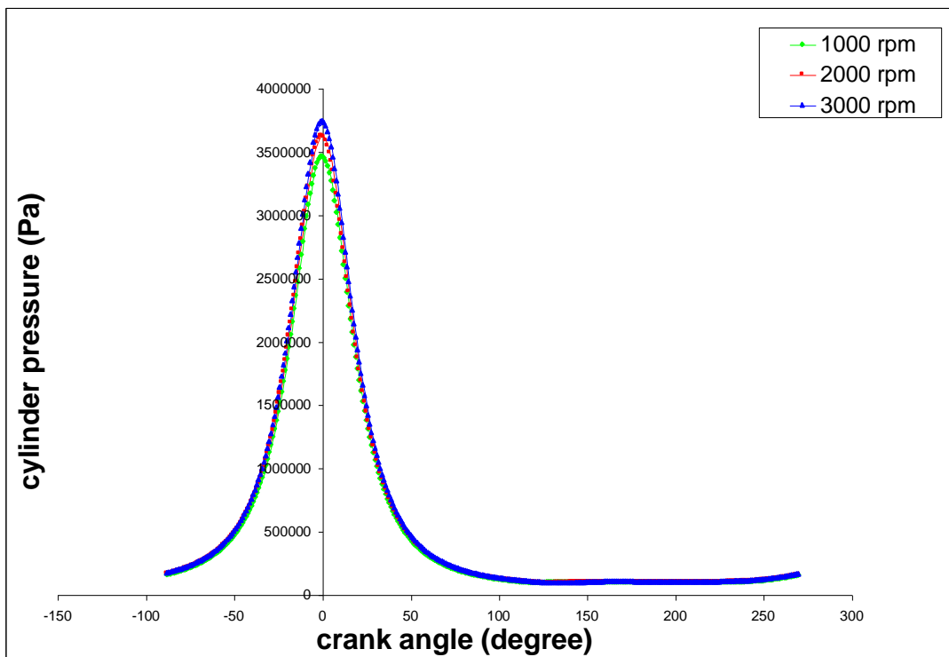
Figure 4: Cylinder pressure profile in motoring test is plotted against the crank angle for 1000, 2000, and 3000 rpm engine speed.
