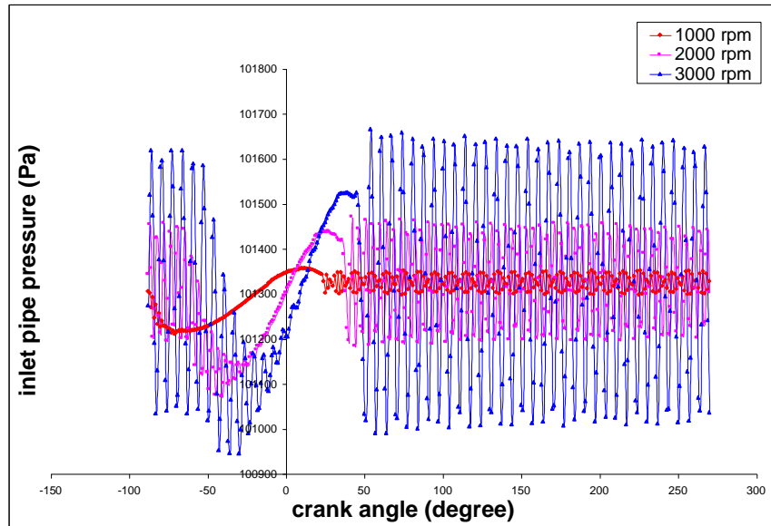
Figure 3: Pressure fluctuation inside the inlet tract prior to the reed valve is plotted against the crank angle for 1000, 2000 and 3000 rpm engine speed.
