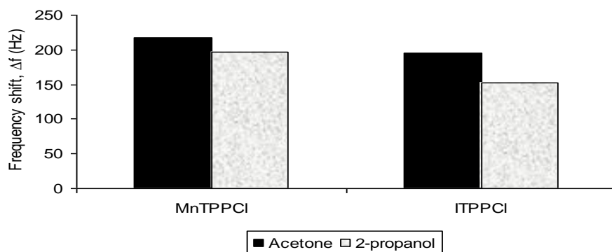
Figure 5: The variation response for acetone and 2-propanol vapors towards MnTPPCL and ITPPCL thin films
