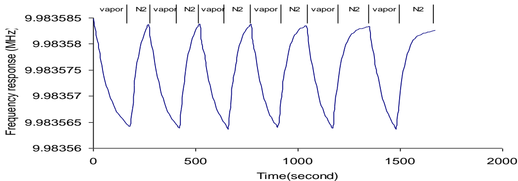
Figure 4: Response of ITPPCl thin film towards acetone vapor
