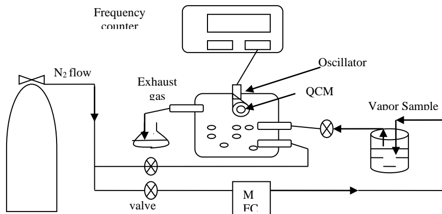
Figure 1: The bulk acoustic system set-up
